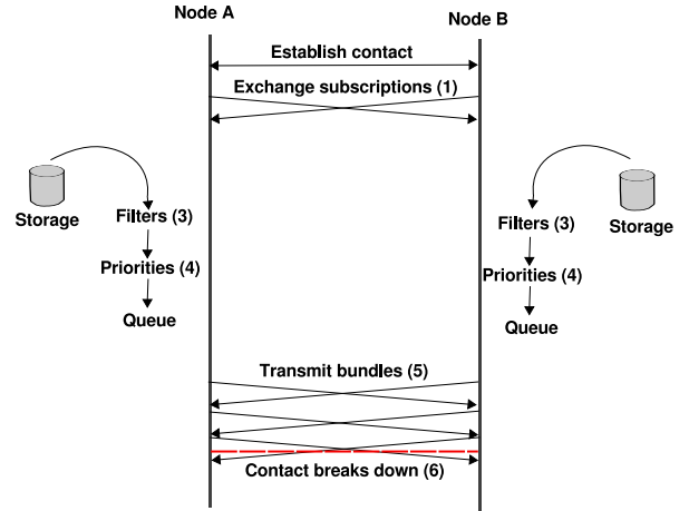
Fig. 2. Contact sequence
